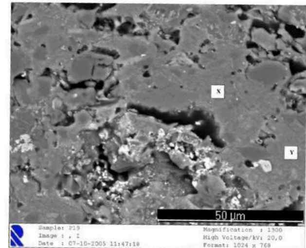
Fig. 3a. SEM micrographs of tungsten mine waste geopolymeric mortar. The areas marked as X and Y are identified as some type of aluminosilicate with the following composition: X [(CaO/SiO 2 = 0); (Al 2 O 3 /Na 2 O eq = 2.5) and (SiO 2 /Al 2 O 3 = 4); Y [(CaO/SiO 2 = 0); (Al 2 O 3 /Na 2 O eq = 3.1) and (SiO 2 /Al 2 O 3 = 3.1).
