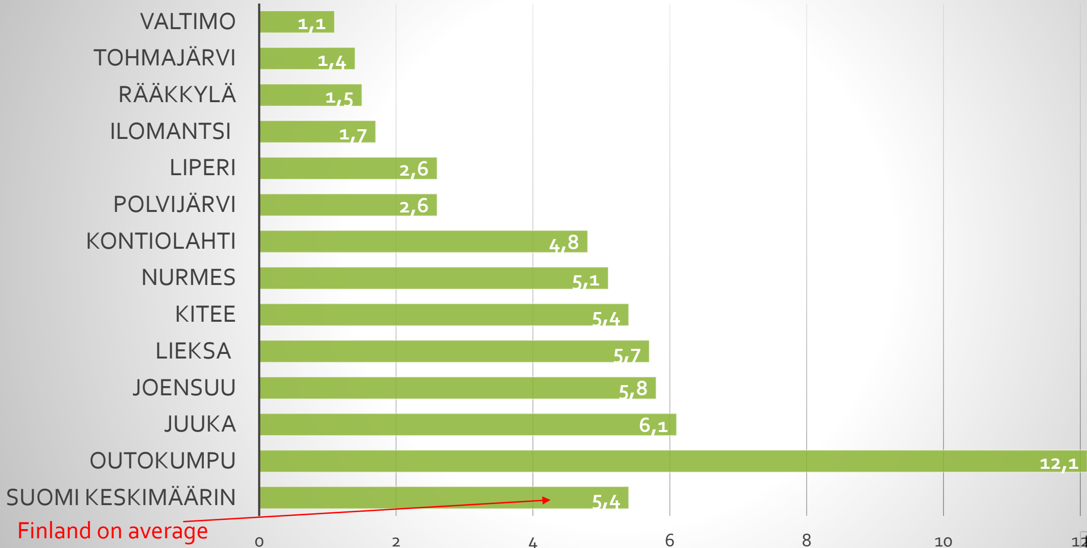
Industrial jobs % of municipality's population (2014/15)
