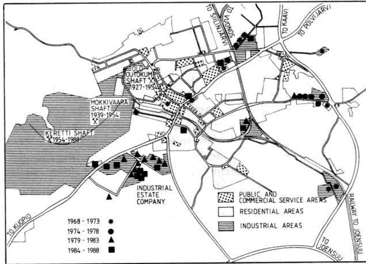
Figure 10.4 Town plan of Outokumpu and years of construction of industrial premises
